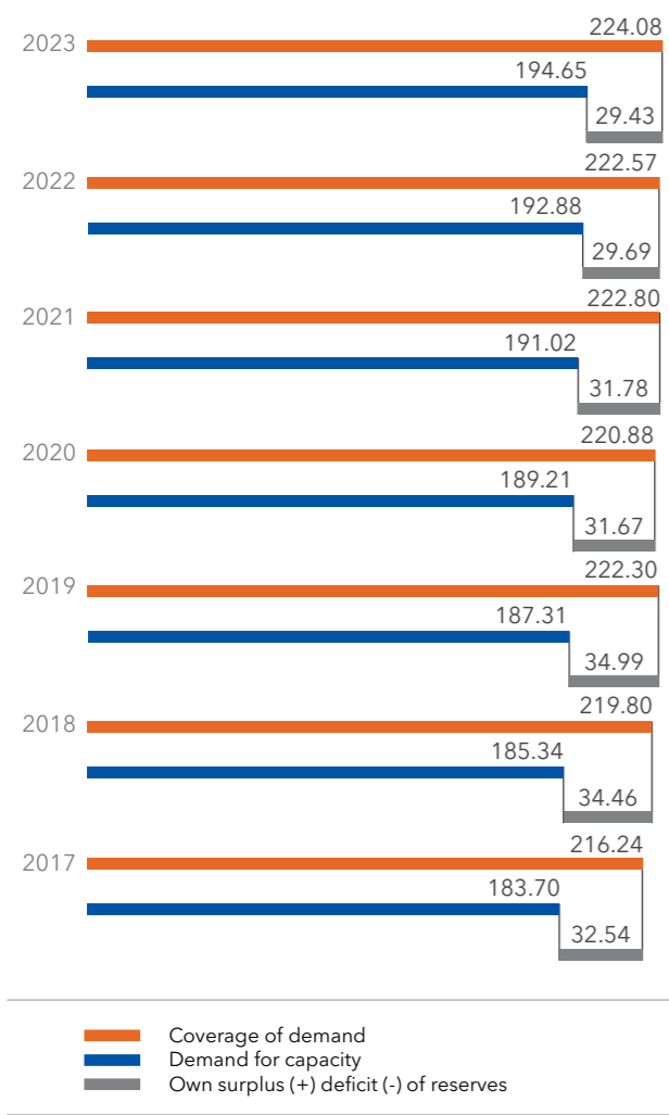
Capacity balances for UES of Russia 2 , GW
